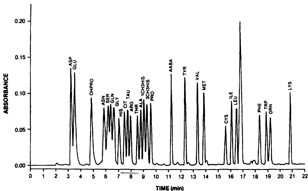
Fig. 4. Elution profile of a 27-amino-acid standard showing resolution of each PTC amino-acid by liquid chromatography (from Ref. [40] with permission). A Pico-Tag amino-acid analysis column (150×3.9 mm I.D.) was used and maintained at 47.5°C. OHPRO=Hydroxyproline; AABA= \alpha -aminobutyric acid; 1CH3HIS and 3CH3HIS=1- and 3-methylhistidine.
