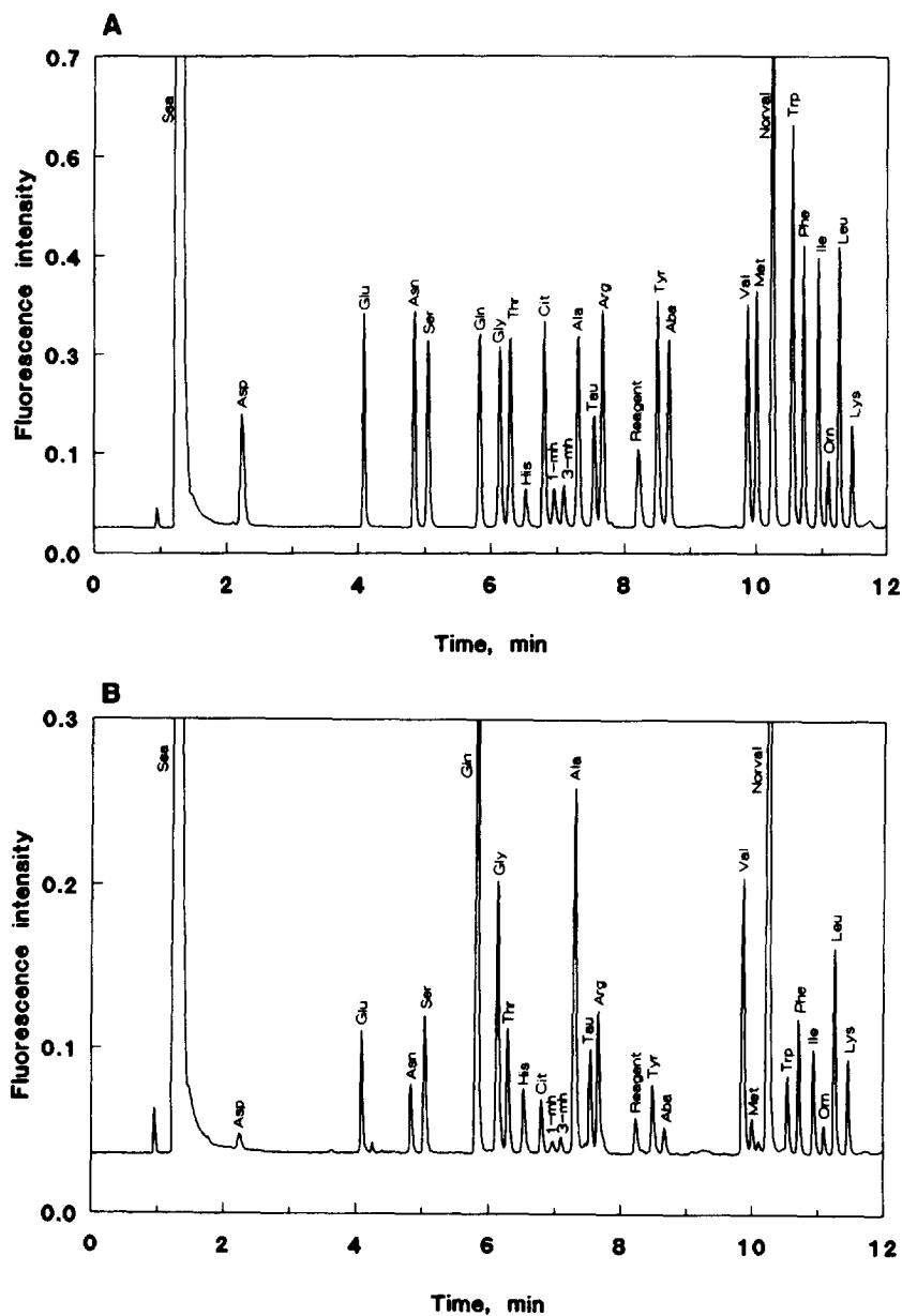
Fig. 1. Elution profile of an OPA-derivatized physiological amino acid standard (A) and a human plasma sample (B) (from Ref. [30] with permission). Column: 3- \mu m Microsphere C s (100 \times 4.6 mm I.D.); flow-rate, 1.5 ml/min; temperature, ambient. Ssa=5-sulphosalicylic acid; 1-mh=1-methylhistidine; 3-mh=3-methylhistidine; Aba= \alpha -aminobutyric acid; Norval= norvaline.
